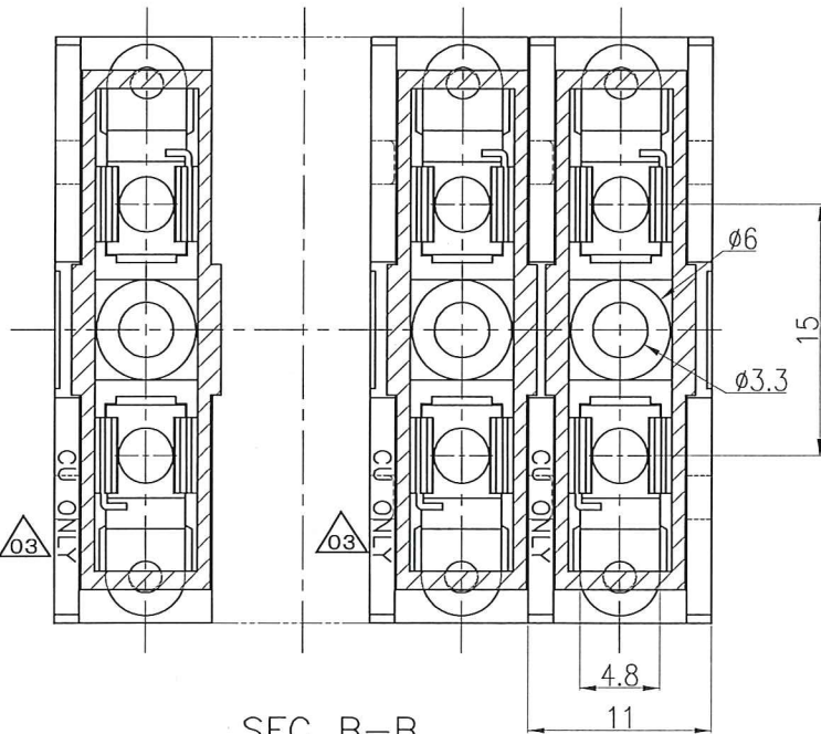
SEC B-B
