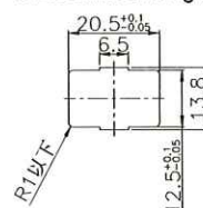
取付穴参考図 Size of mounting hole
