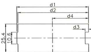
取付穴参考図 Size of mounting hole
