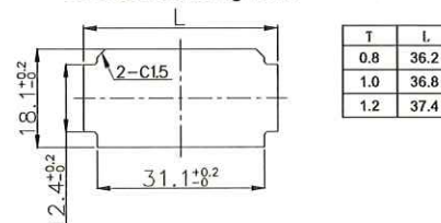
取付穴参考図 Size of mounting hole
