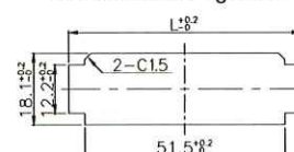
取付穴参考図 Size of mounting hole
