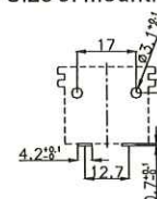
取付穴参考図 Size of mounting hole
