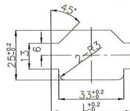
取付穴参考図 Size of mounting hole
