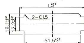
取付穴参考図 Size of mounting hole
