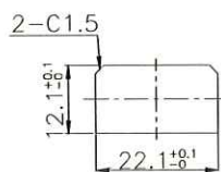
取付穴参考図 Size of mounting hole
