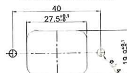
取付穴参考図 Size of mounting hole
