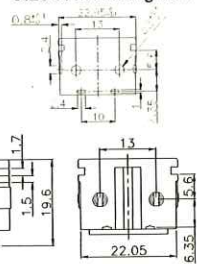
取付穴参考図 Size of mounting hole
