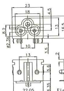
取付穴参考図 Size of mounting hole
