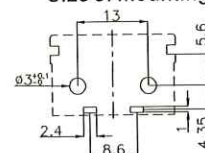
取付穴参考図 Size of mounting hole
