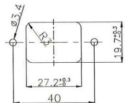
取付穴参考図 Size of mounting hole
