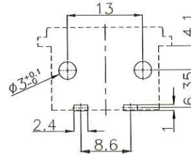
取付穴参考図 Size of mounting hole
