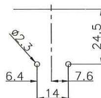
取付穴参考図 Size of mounting hole
