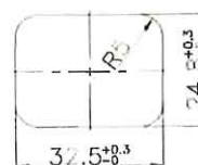
取付穴参考図 Size of mounting hole
