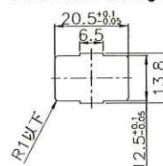
取付穴参考図 Size of mounting hole
