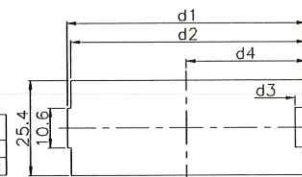
取付穴参考図 Size of mounting hole
